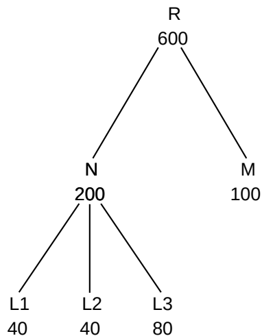
Linux htb
