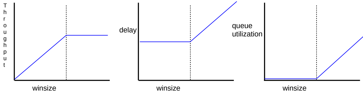
Graphs of winsize versus throughput, delay and queue utilization. Vertical dashed line represents winsize = bandwidth x no-load delay
