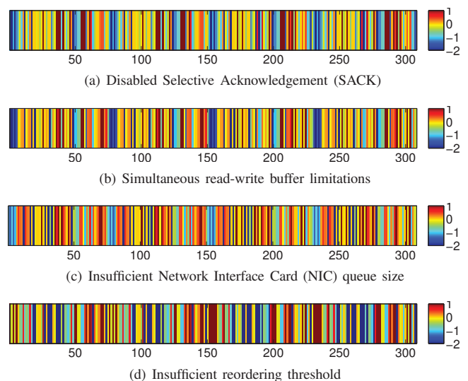
Fig. 1. Comparison of NSSs for four common soft-failures in EUDs. Here, the normalized value of 300 features have been scaled (1 \leftrightarrow -2) and then color coded for easy visualization and comparison. The combination of features uniquely represent each fault and can be used as a “fingerprint” for problem diagnosis.
